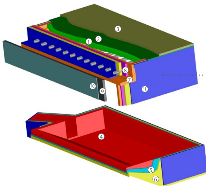
Cross-section of an electrical heating holding furnace
